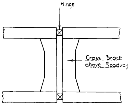
Fig. 143.—Plan at Crown.
